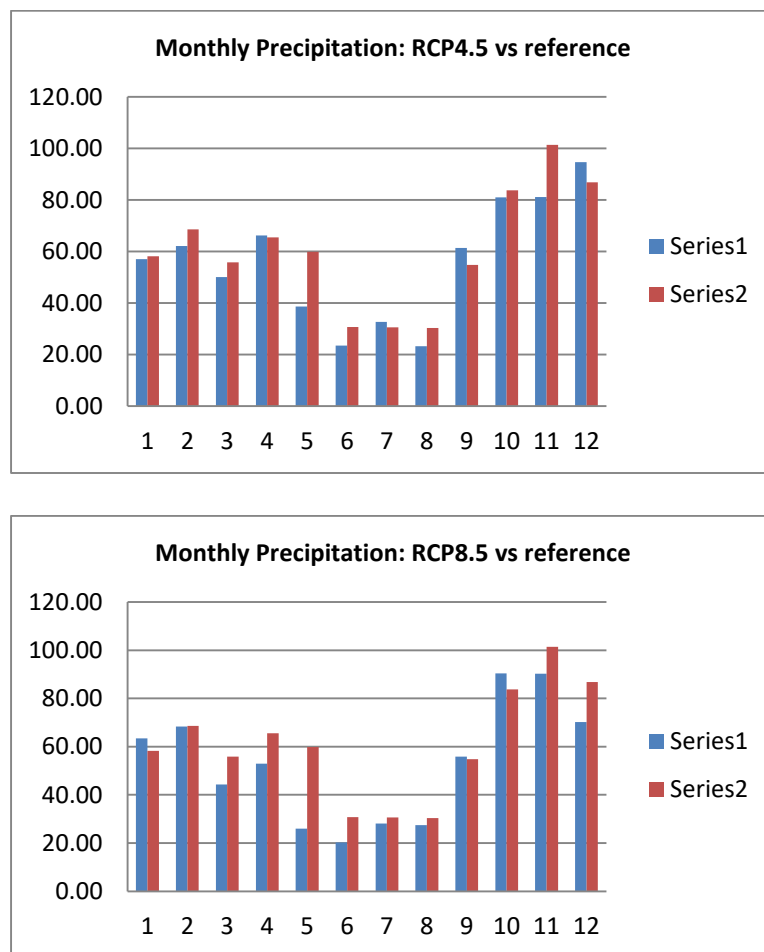
Figure 1 Monthly precipitation RCP4.5 / 8.5 scenarios (2071-2100) vs reference period (1971-2000)
