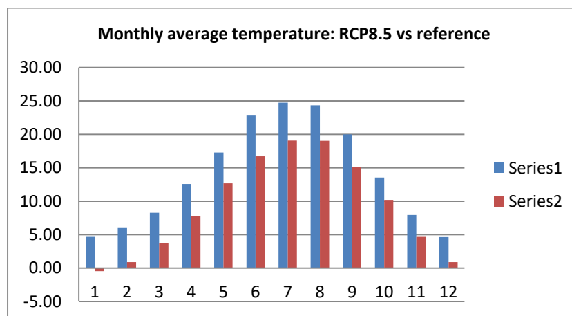
Figure 2 Monthly average temperature: RCP4.5 / 8.5 scenarios (2071-2100) vs reference period (1971-2000)
