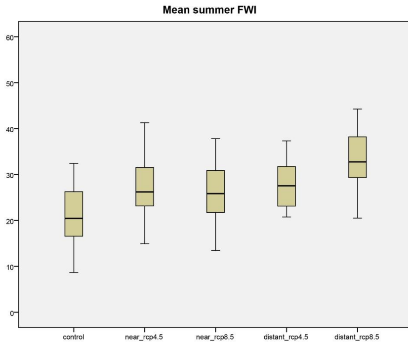
Figure 7.3: Box and whisker plots for mean summer FWI for Prespa for the control period (1971-2000) as well as the near (2031-2060) and distant (2071-2100) future under RCP4.5 and 8.5.
